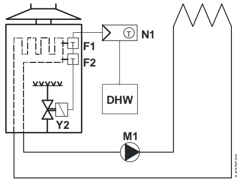
Room thermostat with direct control of a gas-fired wall-hung boiler and independent control of DHW
